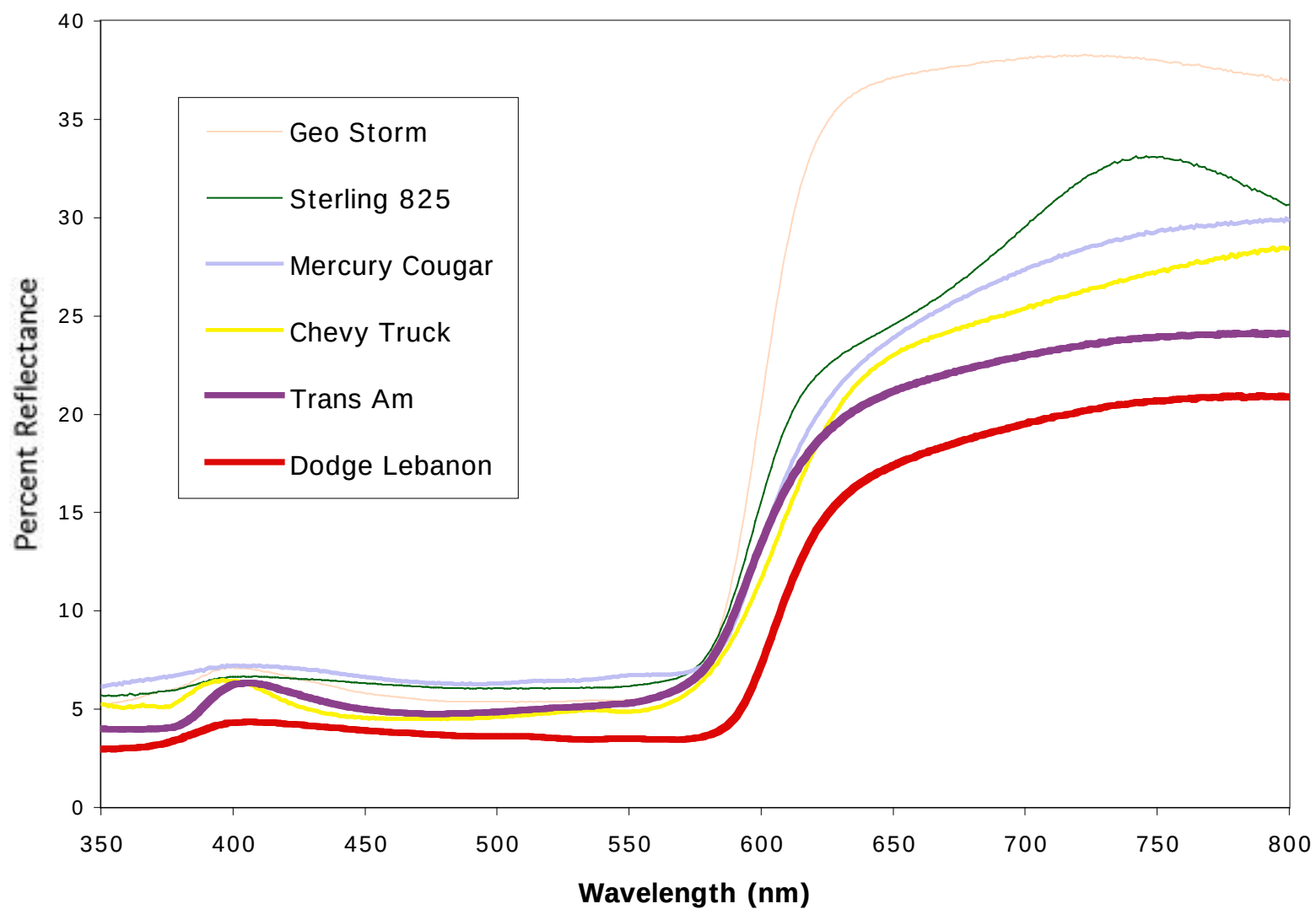
Visible Reflectance Spectra of Red Paints
