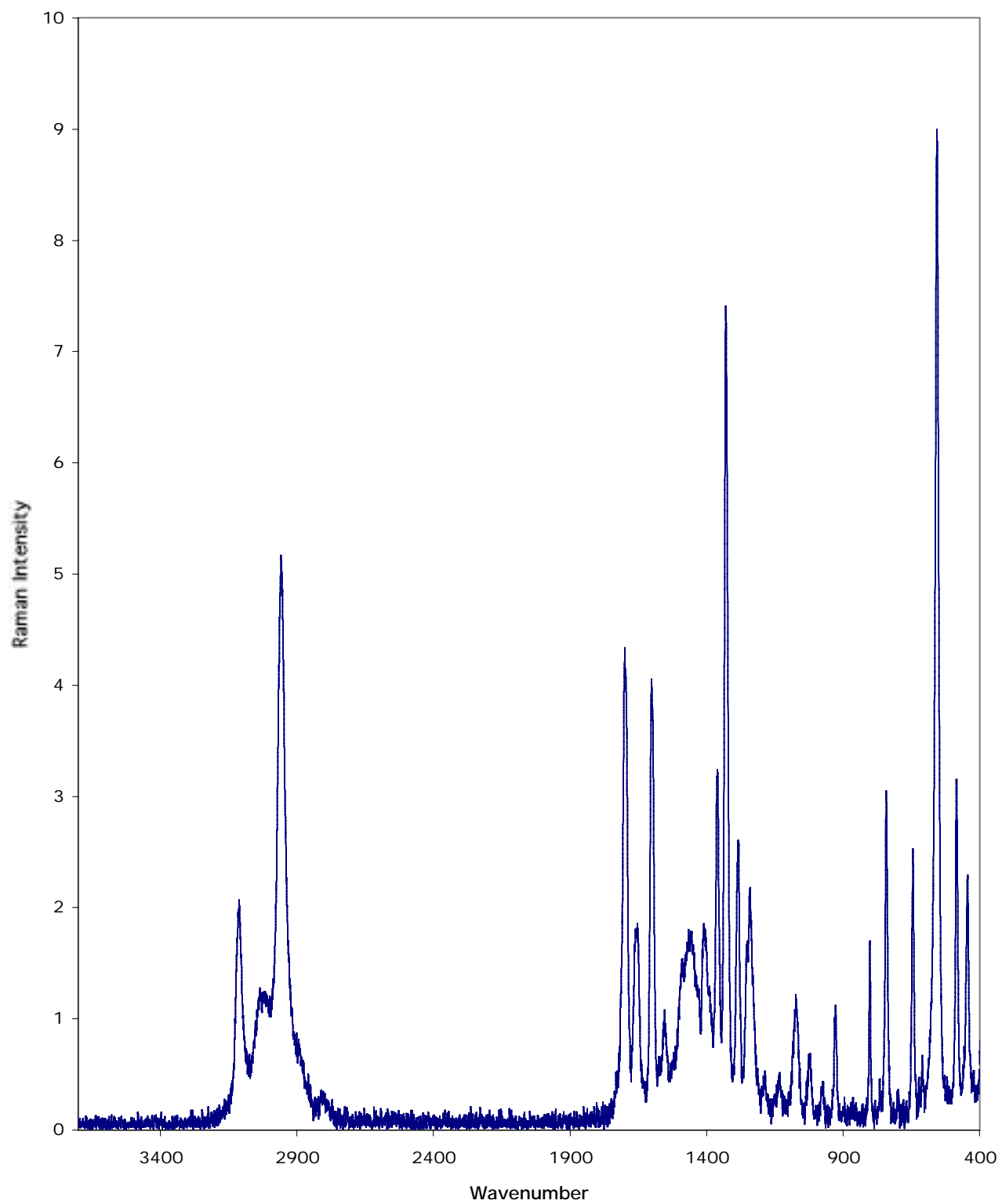
FT-Raman Spectrum of "Cocaine" (caffeine)
